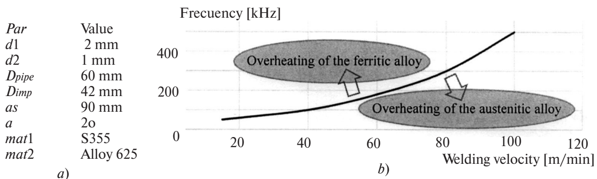
Fig. 4. Geometrical and material parameter set for single frequency simulation (a), frequency – welding velocity curve for convenient welding temperature at the join edge
