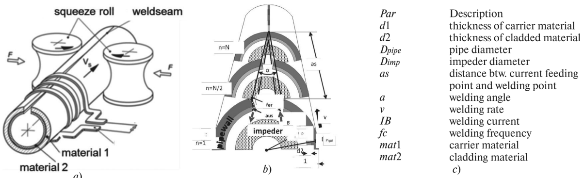
Fig. 1. Overview of inductive pipe welding process (a), 2D model steps along the pipe edge move (b) and model parameters considered by the simulation (c)
