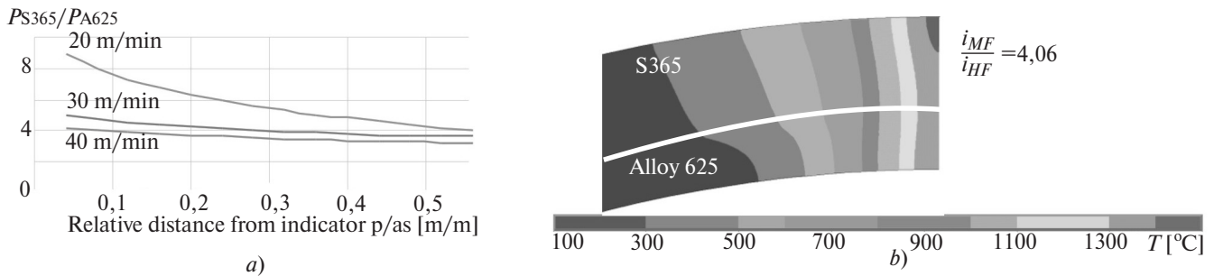
Fig. 5. Total power proportion between the layers for different welding velocities (a), resulting temperature distribution for the welding velocity of v = 40 m/min
