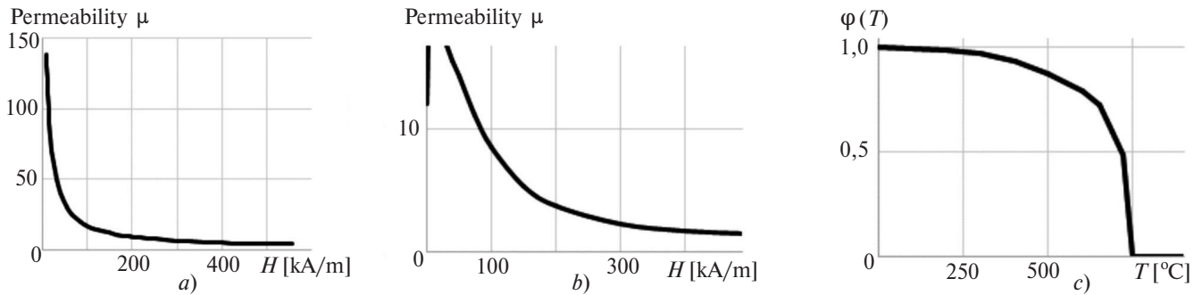
Fig. 3. Magnetic field dependent permeability of S355 at 20°C (a), permeability of the ferrite impeder (b) and temperature dependent function of permeability \varphi(T) referring to [15, p. 76] (c)
