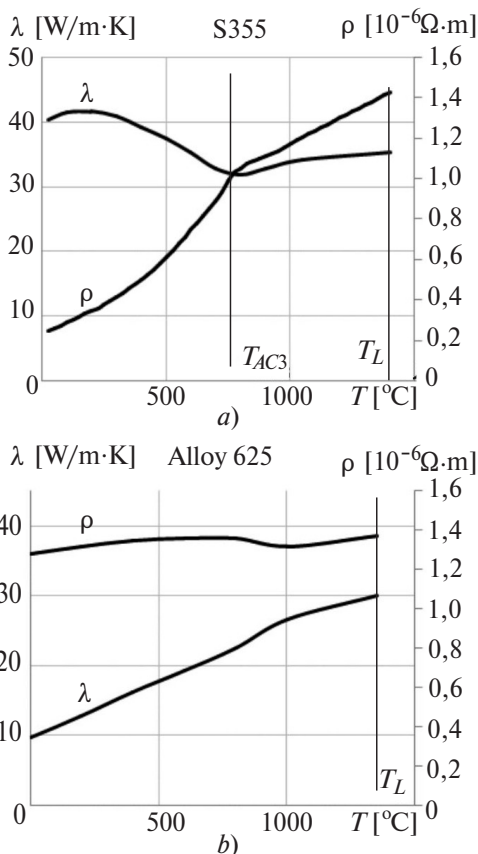
Fig. 2. Specific electrical resistance \rho and thermal conductivity \lambda of S355 (a) and Alloy 625 (extrapolated to the melting points) (b)
